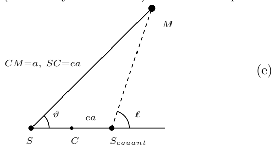
Fig. (e): The equant construction of Ptolemy adapted to a heliocentric theory of Mars; S is the Sun, M is Mars, C the center of the orbit and the equant point is S_{equant} .
