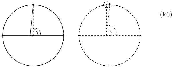
Fig. (k6): Fabricius' (left) and Kepler's (right) deferents, epicycles and ellipses with eccentricity e = 0.1 . On the drawing scale one neither appreciates the difference between ellipse and the deferent circles nor the epicycle in the first drawing. The solid line and dashed lines (indistinguishable in the picture) are respectively the ellipse and the deferent
