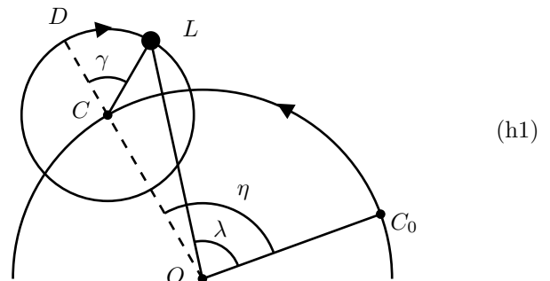
Fig. (h1): Hipparchus' lunar theory: deferent and epicycle.
