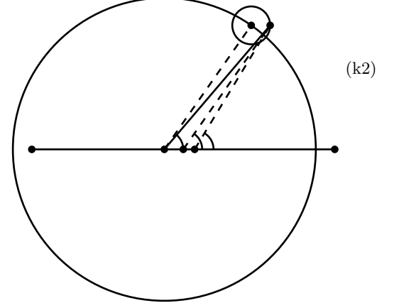
Fig. (k2): Same as Fig. (k1) with eccentricity e = 0.1 ; only the deferent and the epicycle are drawn. The actual orbit (not drawn) is the circle with the horizontal segment as a diameter
