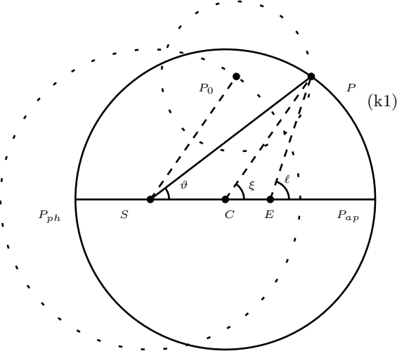
Fig. (k1) The vicarious hypothesis: here the eccentricities are e = \frac{5}{4}0.4 and e' = \frac{3}{4}0.4 , \sim 4 times larger than real to make a clearer picture. The dashed circles are the deferent (centered at S ) and the epicycle (centered at P_0 ) while the planet is in P . The continuous circle is the actual orbit. The segment SP_0 is parallel to CP (partially drawn) so that PCP_{ap} = P_0SP_{ap} is the eccentric anomaly \xi while PSP_{ap} is the true anomaly \vartheta and PEP_{ap} is the average anomaly \ell , that rotates uniformly around the equant E .
