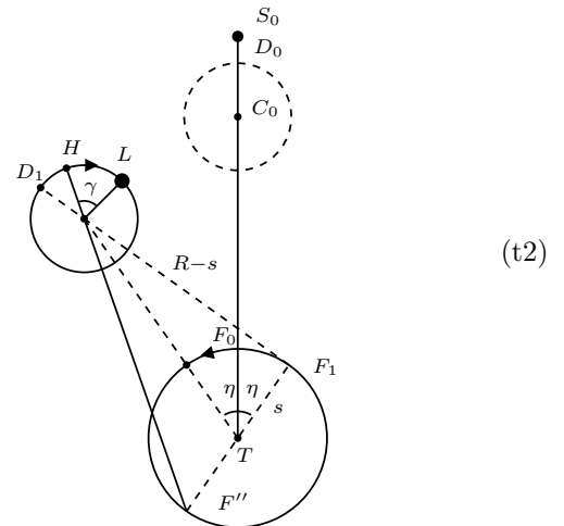
Fig. (t2): The more refined theory of Ptolemy
