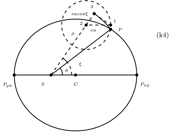
Fig. (k4): Kepler’s construction of the ellipse. The eccentricity is e = 0.4 to make a clearer drawing. The planet is in P . The segment 23 is the projection on S3 of the segment 31 and the segment SP is equal to S3 . The epicycle (dashed circle) is no longer holding the planet but it determines its position. The anomaly \xi is the anomaly of the center of the epicycle. Motion verifies the law \rho \dot{\xi} = \text{const} .
