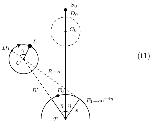
Fig. (t1): Ptolemy's correction to Hipparchus' lunar theory.
