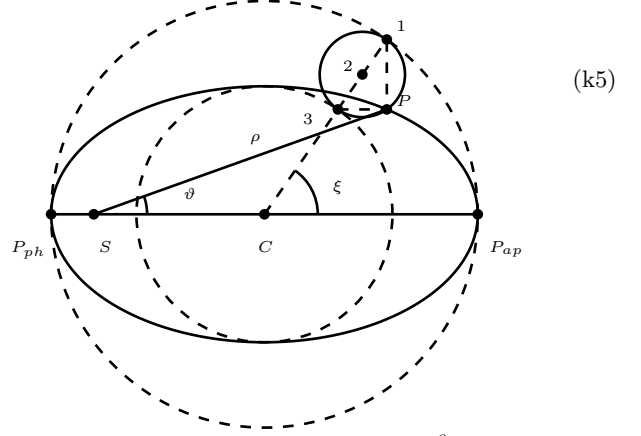
Fig. (k5): Fabricius’ interpretation, see 3 p. 402-403, of Kepler’s ellipse. The ellipse has very high eccentricity ( e = 0.8! ) to make visible the small epicycle. The planet is in P and C3 = b , C1 = a and the center of the epicycle is 2 . Eccentric anomaly reckoned at C and the angle 12P is 2\xi
