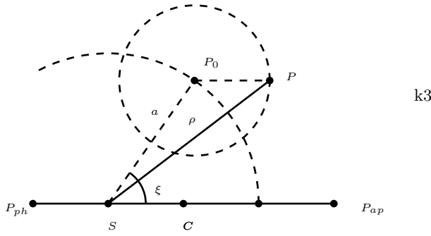
Fig. (k3): The first attempt to establish the law \rho \dot{\xi} = \text{const} . Eccentricity ( e = 0.4 ) is much larger than the real value, for illustration purposes. The deferent is a circle of radius a around S and the epicycle of radius ea is centered at P_0 , with anomaly \xi with respect to S , the planet is in P
