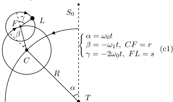
Fig. (c1): Copernicus’ lunar theory with two epicycles
